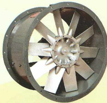
VARIABLE PITCH AXIAL FLOW FAN
